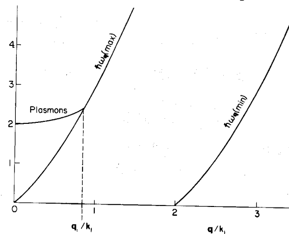
Fig. 9.3 Spectrum of excitations for a free-electron gas. A collective plasma mode splits off from the continuum of single electron excitations below a critical wave vector q_c . In this illustration, \hbar\omega_p has been taken equal to twice the Fermi energy, hence \hbar\omega_p = \hbar^2 k_F^2 / m .
