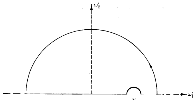
Fig. 6.1 Integration contour for obtaining Eq. (6.14).
