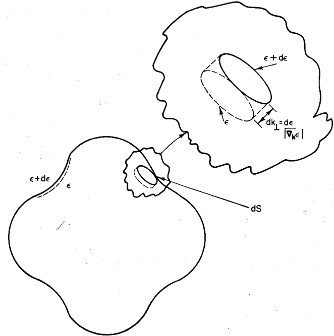
Fig. 5.4 Element of area dS on a constant-energy surface in \mathbf{k} -space. The element of volume between two surfaces of constant energy \mathcal{E} and \mathcal{E} + d\mathcal{E} is seen from the insert to be dV = dS d\mathcal{E} / |\nabla_{\mathbf{k}} \mathcal{E}| .
