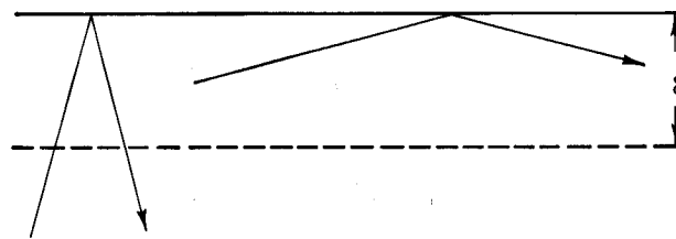
Fig. 4.5 Electron trajectories near the surface. Only electrons traveling nearly parallel to the surface are effective in absorbing and screening electromagnetic radiation when l \gg \delta .
