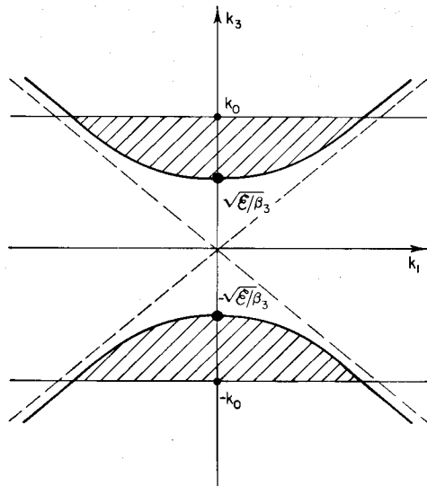
Fig. F.3 Section of paraboloids showing region of integration.
