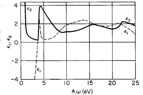
Fig. 3.17 Spectral dependence of the real and imaginary dielectric functions for Ag. [From H. Ehrenreich and H. R. Philipp, Phys. Rev. 128, 1622 (1962).]
