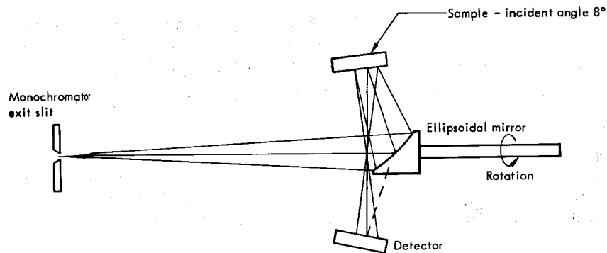
Fig. 1.3 Schematic of optical system for near-normal-incidence reflectivity measurements. The arrangement reduces the number of reflections to one. This is an important and valuable feature in the vacuum-ultraviolet, where the reflectance of solids is low and the use of a multiple-reflection scheme drastically reduces light intensity. The ellipsoidal mirror diverts the light beam consecutively onto the sample and the detector. Continuous rotation thus produces a sequence of "incident" and "reflected" pulses which are electronically measured and recorded. [From T. Huen, G. B. Irani, and F. Wooten, Appl. Opt. 10, 552 (1971).]
