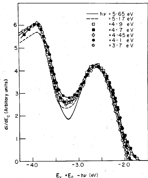
Fig. 5.36 Energy distributions for \text{Cs}_3\text{Bi} plotted versus the energy in the valence band \epsilon_v , from which the electrons are excited. This is done by subtracting the photon energy h\nu from the external kinetic energy of the photoelectrons. Energy is measured from the vacuum level. The values of h\nu indicate the energy of the incident radiation. [From W. E. Spicer, Phys. Rev. Lett. 11, 243 (1963).]
