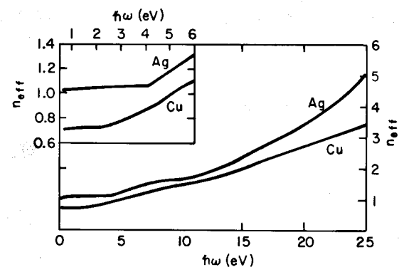
Fig. 5.12 Effective numbers of electrons per atom contributing to the optical properties over a given energy range versus energy. [From H. Ehrenreich and H. R. Philipp, Phys. Rev. B1 , 1622 (1962).]
