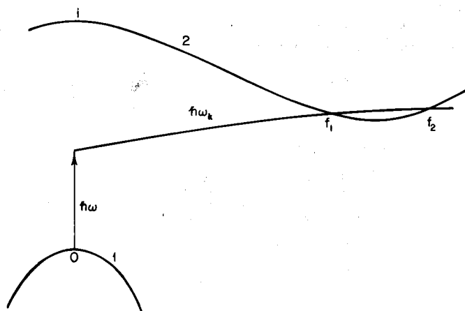
Fig. 5.22 The energy conditions for an indirect transition. (1) Valence band, (2) conduction band. The phonon dispersion curve \hbar\omega_k is superposed on the electronic band diagram so as to show the final states reached by a combination of photon and phonon absorption. The energy scale for the phonon dispersion curve is exaggerated. Note that the end of the arrow indicating photon absorption does not correspond to the intermediate state for the overall indirect transition. It merely indicates the amount of energy contributed by the photon. The true intermediate state is indicated by i .
