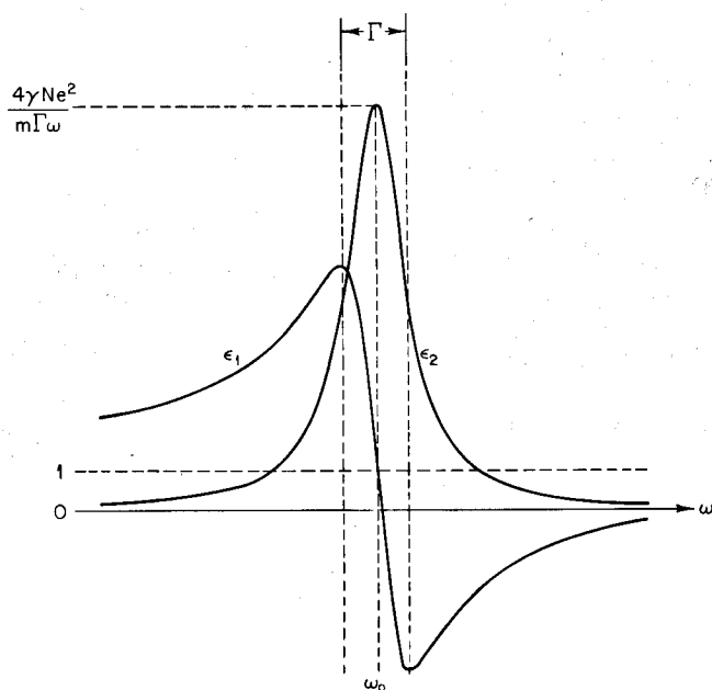
Fig. 3.1 Frequency dependence of \epsilon_1 and \epsilon_2 .
