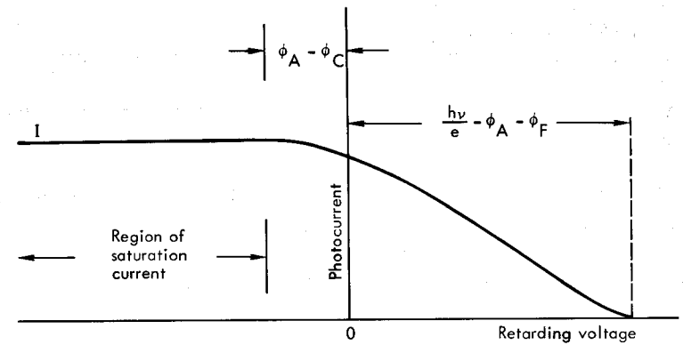
Fig. 1.12 Photocurrent versus retarding voltage for the semiconductor photocathode and metal anode of Fig. 1.11. The cutoff voltage differs from that for a metal photocathode by \phi_F , the Fermi potential measured with respect to the valence band maximum.
