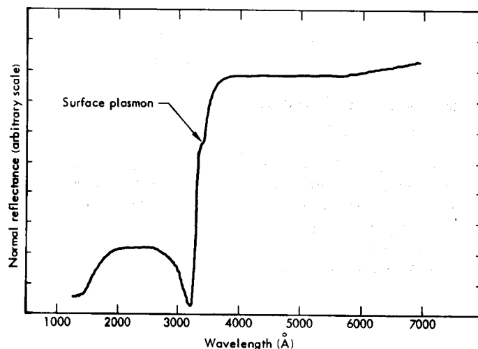
Fig. 9.7 Normal-incidence reflectance for an unannealed film of silver. The dip in reflectance at 3400 \text{ \AA} arises from surface plasmon excitation made possible by surface roughness. This dip in reflectance is not present in the annealed film (same sample) shown in Figs. 3.15 and 5.14. [From T. Huen, G. B. Irani, and F. Wooten, Appl. Opt. 10, 552 (1971).]
