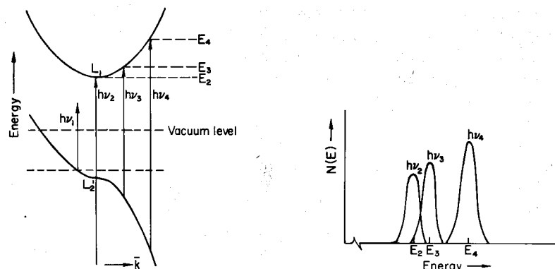
Fig. 5.34 Direct transitions in copper and their contributions to photoemission. The important feature of the peak is that it moves to higher energy at a somewhat slower rate than the increase in photon energy. Note that E_3 - E_2 \neq hv_3 - hv_2 and E_4 - E_3 \neq hv_4 - hv_3 . [From C. N. Berglund and W. E. Spicer, Phys. Rev. 136, A1030 (1964).]
