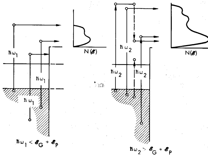
Fig. 5.38 Left: A hypothetical EDC for a semiconductor with \hbar\omega_1 < \varepsilon_G + \varepsilon_p , where \varepsilon_p is the threshold energy for pair production. Here, the only electrons escaping are those which have suffered no scattering or only nearly elastic scattering. The structure in the EDC is characteristic of that in the initial optical excitation. Right: An EDC for photon energy \hbar\omega_2 > \hbar\omega_1 such that \hbar\omega_2 > \varepsilon_G + \varepsilon_p . Some electrons can escape even after having suffered large energy losses. These electrons contribute to a low-energy peak which often consists mostly of scattered electrons. The peaks at higher energy contain few scattered electrons and thus are representative of the structure in the initial optical excitation.
