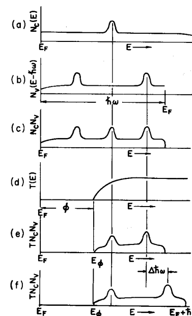
Fig. 5.33 Relationship between density of states (taken from Fig. 5.32) and photoelectron energy distribution for indirect transitions with constant matrix elements. (a) Conduction band (empty), (b) valence band (filled), (c) photoexcited electrons, (d) escape function, (e) photoemitted electrons ( \hbar\omega ), (f) photoemitted electrons ( \hbar\omega' ). [From A. J. Blodgett, Jr. and W. E. Spicer, Phys. Rev. 146 , 390 (1966).]
