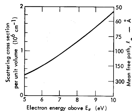
Fig. 5.41 Calculated cross section and mean free path for electron-electron scattering in Al. The mean free path for electron-phonon scattering was taken as 200 Å. [From T. Huen and F. Wooten, Solid State Commun. 9, 871 (1971).]
