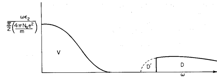
Fig. 3.28 Absorption versus frequency for a metal like Cd. [After N. V. Smith, Advan. Phys. 16, 629 (1967).]
