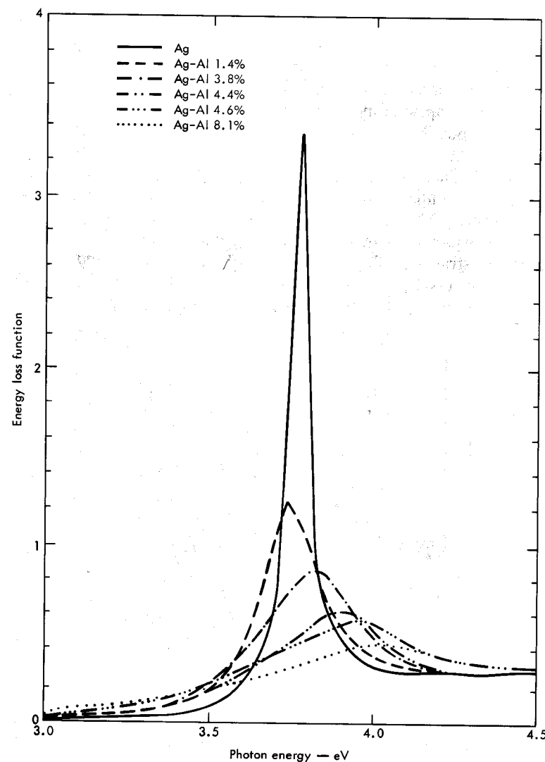
Fig. 5.17 The energy loss functions versus photon energy for Ag and Ag-Al alloys at 300°K. [From G. B. Irani, T. Huen, and F. Wooten, Phys. Rev. 3B , 2385 (1971).]
