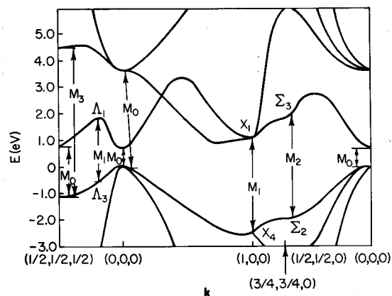
Fig. 5.8 The band structure of Ge. [From J. C. Phillips, D. Brust, and G. F. Bassani, Proc. Int. Conf. Phys. Semicond. Exeter London p. 564 (1962).]
