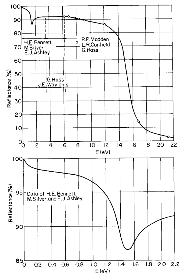
Fig. 3.13 Reflectance of aluminum. The decrease in reflectance at \hbar\omega = 1.4 eV arises from a weak interband transition. The large decrease in reflectance at \hbar\omega = 14.7 eV identifies the plasma resonance. [From H. Ehrenreich, H. R. Philipp, and B. Segall, Phys. Rev. 132 , 1918 (1963).]
