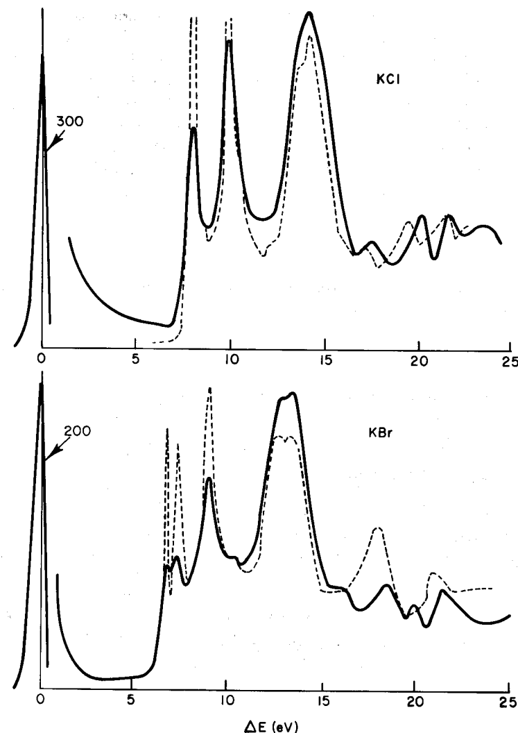
Fig. 9.5 Characteristic energy loss spectra of 50-keV electrons for KCl and KBr. The broken lines represent optical measurements of -\text{Im}(1/\epsilon) . [From M. Creuzburg and H. Raether, Solid State Commun. 2 , 345 (1964).]
