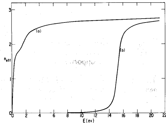
Fig. 3.29 The effective number of electrons per Al atom versus \hbar\omega obtained from a numerical integration of the experimental values of (a) \epsilon_2 and (b) -\operatorname{Im} \epsilon^{-1} . [H. Ehrenreich, H. R. Philipp, and B. Segall, Phys. Rev. 132 , 1918 (1963).]
