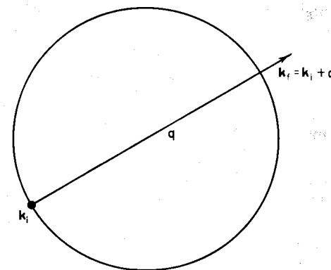
Fig. 9.2 A transition of minimum energy for q > 2k_F . The initial state \mathbf{k}_i lies on the Fermi surface. The final state \mathbf{k}_f is antiparallel to \mathbf{k}_i and lies outside the opposite surface.
