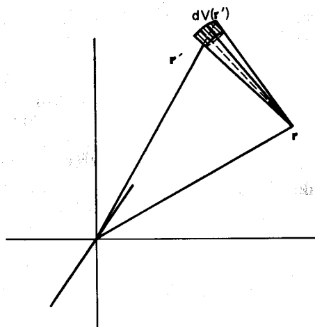
Fig. 4.6 The volume element dV(r') represents a general region in which some electrons are scattered and then travel to r without suffering further collisions.
