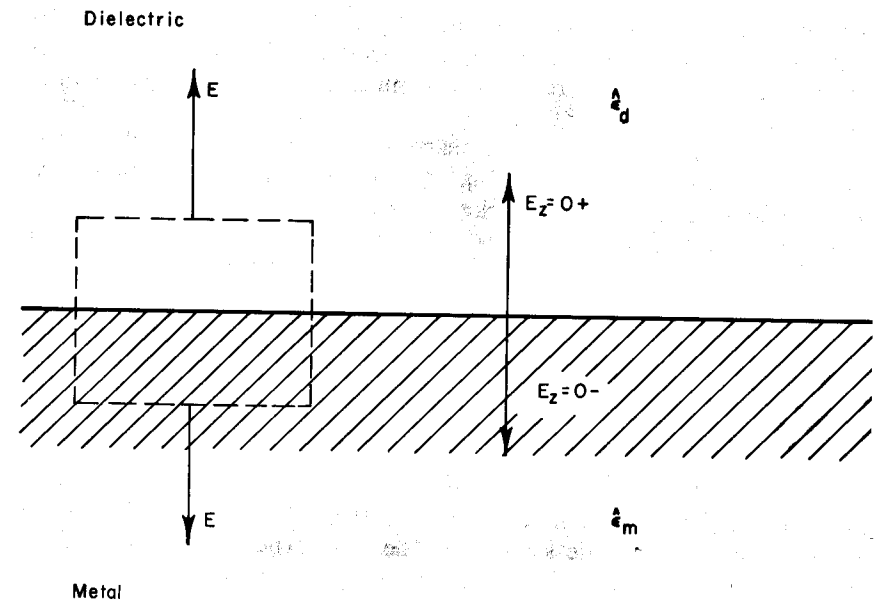
Fig. 9.6 Boundary condition at a metal-dielectric interface in the absence of external charge. The electric field arises only from surface polarization charge and, by symmetry, is of the same magnitude but opposite sign on opposite sides of the interface.
