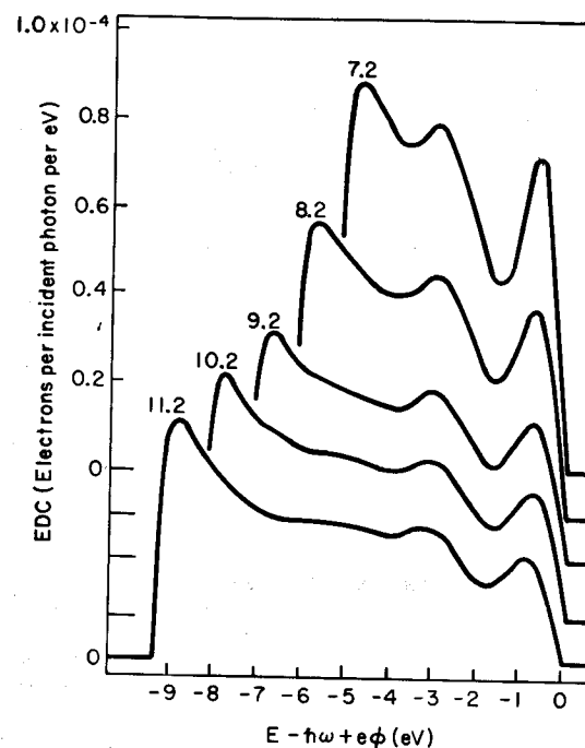
Fig. 9.8 Photoelectron distribution curves for Cs plotted versus the energy of the initial state for unscattered electrons. The zero of energy is thus the Fermi energy. The peak at -3 \text{ eV} arises from excitation of a surface plasmon by an escaping photoelectron. Values given on the various curves are \hbar\omega in electron-volts. [From N. V. Smith and G. B. Fisher, Phys. Rev. 3, 3662 (1971).]
