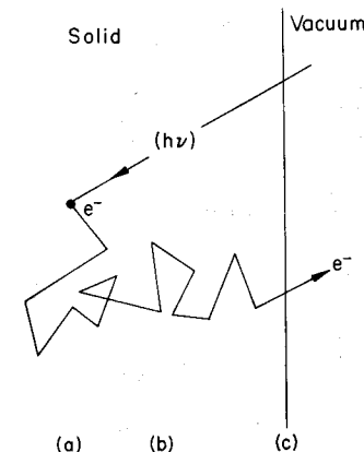
Fig. 1.6 (a) Photoexcitation of an electron, (b) random motion through the crystal, (c) and electron escape. [From W. E. Spicer and F. Wooten, Proc. IEEE 51 , 1119 (1963).]
