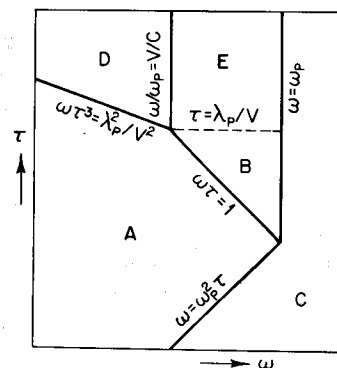
Fig. 4.3. A logarithmic plot of the \omega - \tau diagram showing the regions illustrated in Fig. 4.2. The new region, region C, is characterized by transmission. [From H. B. G. Casimir and J. Ubbink, Philips Tech. Rev. 28 , 300 (1967).]
