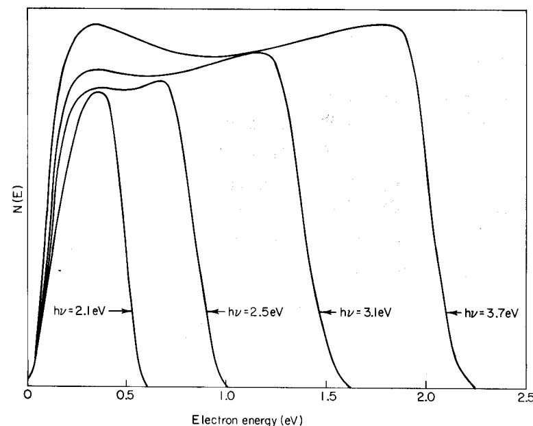
Fig. 3.24 Photoemission from Cu with a surface monolayer of Cs. At photon energies less than 3.7 eV, electrons excited from d states cannot escape. Thus these curves represent electrons excited from s- and p-like states as illustrated in Fig. 3.23. [From C. N. Berglund and W. E. Spicer, Phys. Rev. 136, A1044 (1964).]
