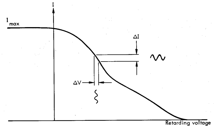
Fig. 1.13 Modulation of I-V curve with small ac voltage permits direct measurement of \Delta I/\Delta V . This is the method used to obtain the energy distribution curve for GaAs shown in Fig. 1.4.
