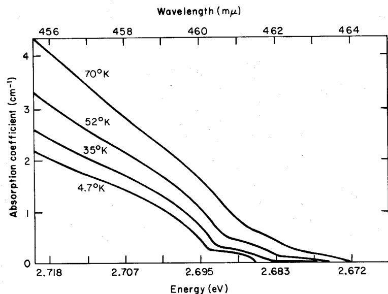
Fig. 5.27 The absorption edge at different temperatures for AgBr containing 1 mole% AgCl. Comparison of this figure with Fig. 5.26 shows that a disorder-induced component sets in exactly halfway between the edges associated with phonon emission and phonon absorption. [From B. L. Joesten and F. C. Brown, Phys. Rev. 148 , 919 (1966).]
