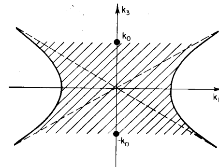
Fig. F.2 A plane through the hyperboloid of Fig. F.1 showing the region of integration.
