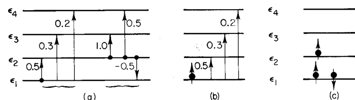
Fig. 3.27 An energy level scheme for a system having only four one-electron energy levels. Possible transitions and oscillator strengths are shown. The oscillator strengths are chosen arbitrarily except for the sum-rule requirement.
