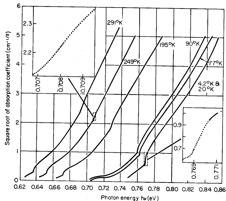
Fig. 5.24 The absorption-edge spectrum of Ge at various temperatures. [From G. G. MacFarlane, T. P. McLean, J. E. Quarrington, and V. Roberts, Phys. Rev. 108 , 1377 (1957).]
