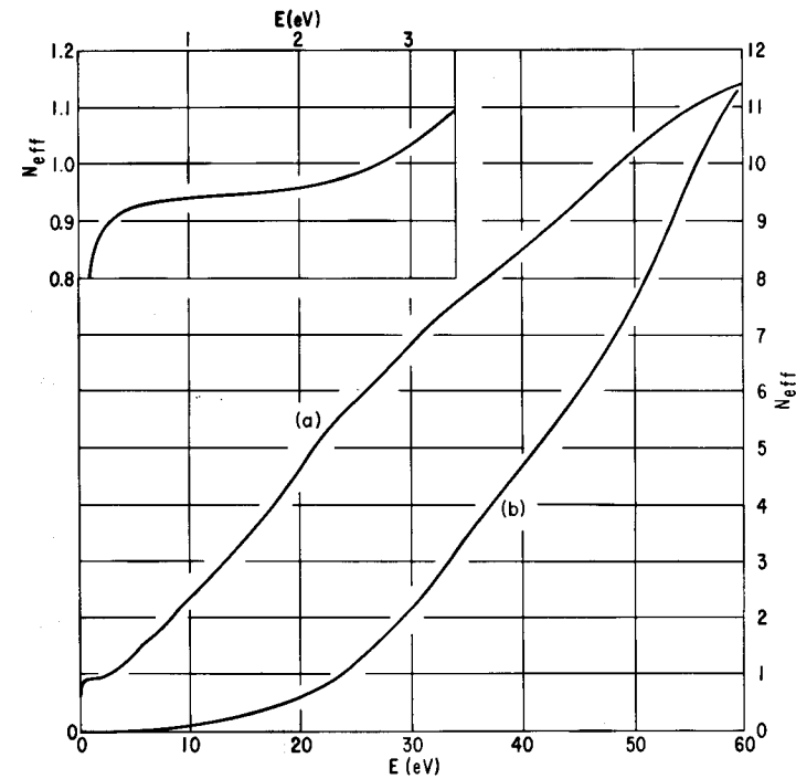
Fig. 3.30 The effective number of electrons per Au atom versus \hbar\omega obtained from a numerical integration of the experimental values for (a) \epsilon_1 and (b) -\operatorname{Im} \epsilon^{-1} . [From B. R. Cooper, H. Ehrenreich, and H. R. Philipp, Phys. Rev. 138 , A494 (1965).]
