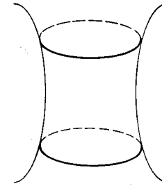
Fig. F.1 A hyperboloid of one sheet.
