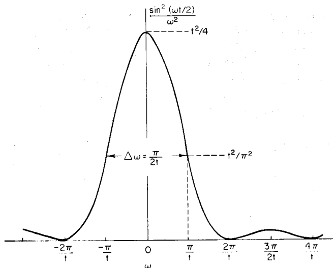
Fig. 5.1 Relative probability of finding an electron excited to a state having an energy \hbar\omega greater than the initial state as determined from first-order perturbation theory.
