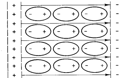
Fig. 3.20 Screening of plasma oscillations by polarization of localized electrons. Compare with Fig. 3.19. The d electrons are highly localized on atomic sites. However, their polarizability may be high enough to cause appreciable screening of the forces between fluctuations in the charge densities of conduction electrons. The result can be a significant shift in the plasma frequency.
