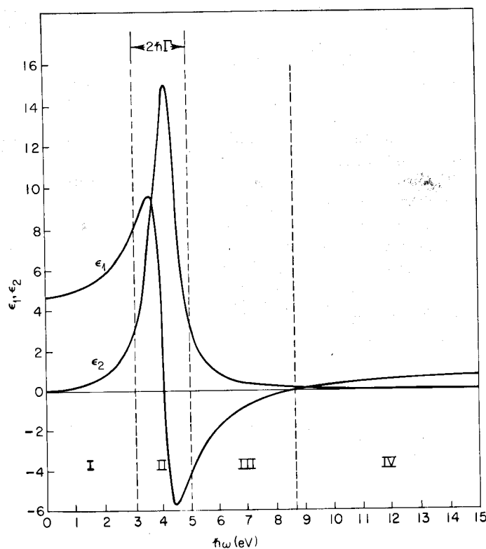
Fig. 3.3 Spectral dependence of \epsilon_1 and \epsilon_2 . The curves are calculated for the case in which h\omega_0 = 4 eV, h\Gamma = 1 eV, and 4\pi Ne^2/m = 60 . The onset of region IV is defined by \epsilon_1 = 0 .
