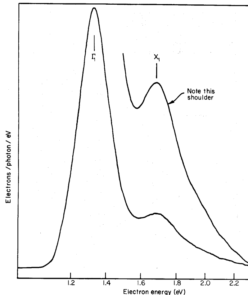
Fig. 5.43 Energy distribution curve for p^+ GaAs: \text{Cs}_2\text{O} for a photon energy of 2.2 eV. [From L. W. James, R. C. Eden, J. L. Moll, and W. E. Spicer, Phys. Rev. 174 , 909 (1968).]
